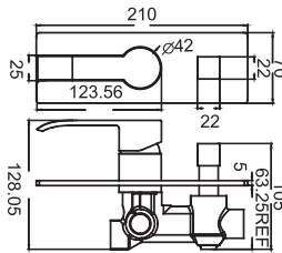
YSW2313-09A Shower mixer with diverter Coating options: Chrome
